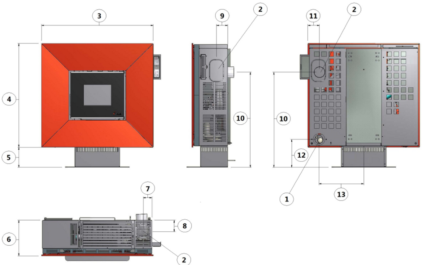
Fig. 14 - General dimensions
