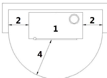
Fig. 18 - Wall mounting
