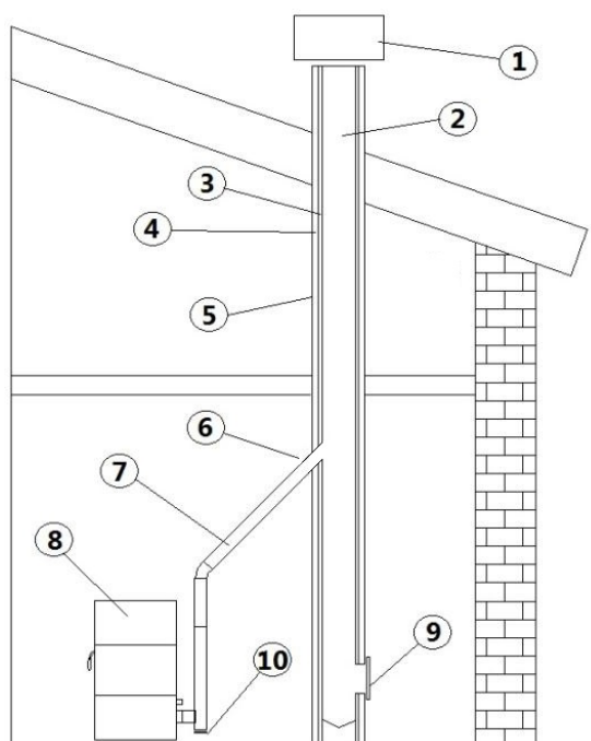
Fig. 5 - Chimney components
