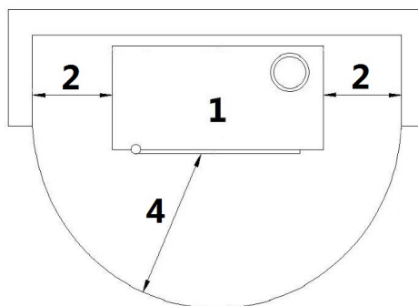
Fig. 18 - Installation murale
