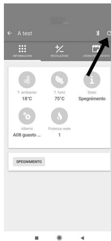
Fig. 34 - Screen refresh
